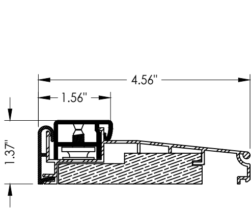
13 INSWING THRESHOLD WORLDWIDE
