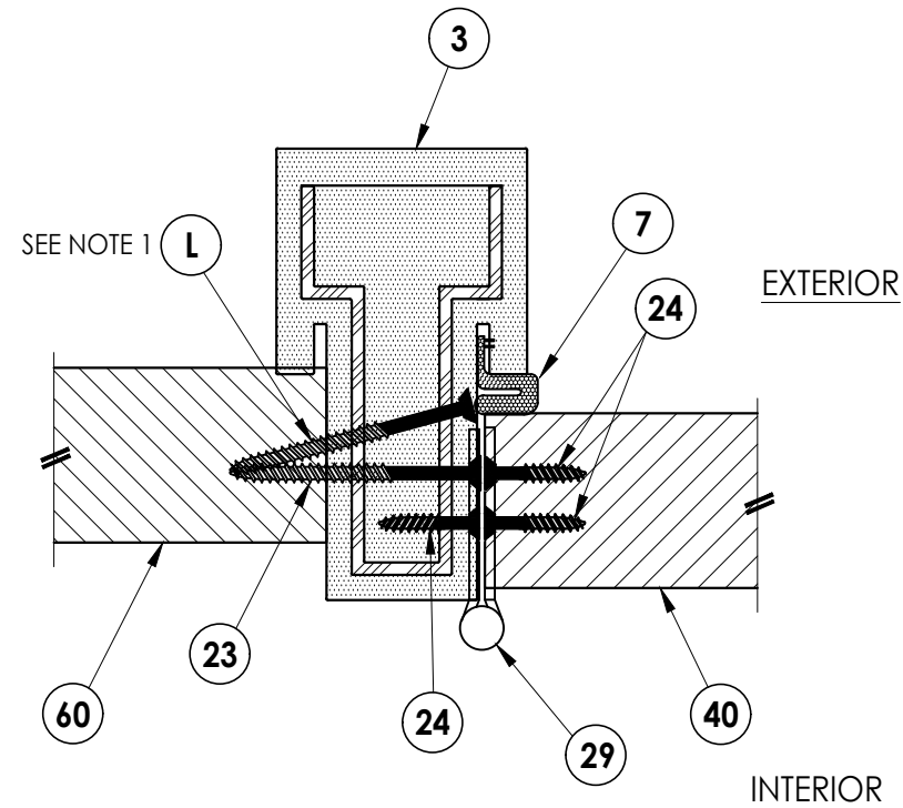
5 HORIZONTAL CROSS SECTION 5 Inswing shown (Outswing similar)
