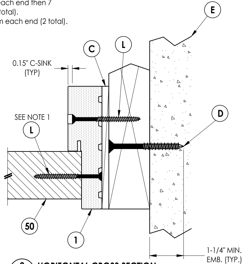
2 HORIZONTAL CROSS SECTION 5 Shown w/ 2X Buck Inswing shown (Outswing similar)
