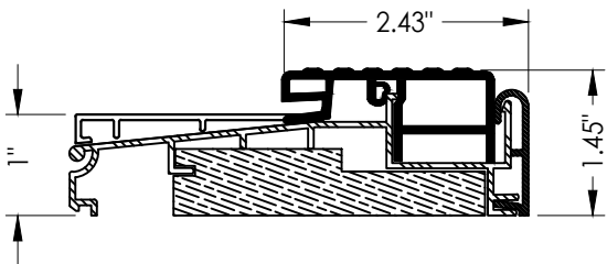
16 OUTSWING THRESHOLD w/ SIDELITE ADAPTER WORLDWIDE
