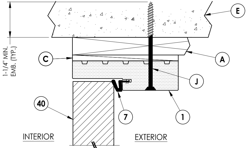
3 VERTICAL CROSS SECTION 6 Shown w/ 1X sub-buck Inswing shown (Outswing similar)
