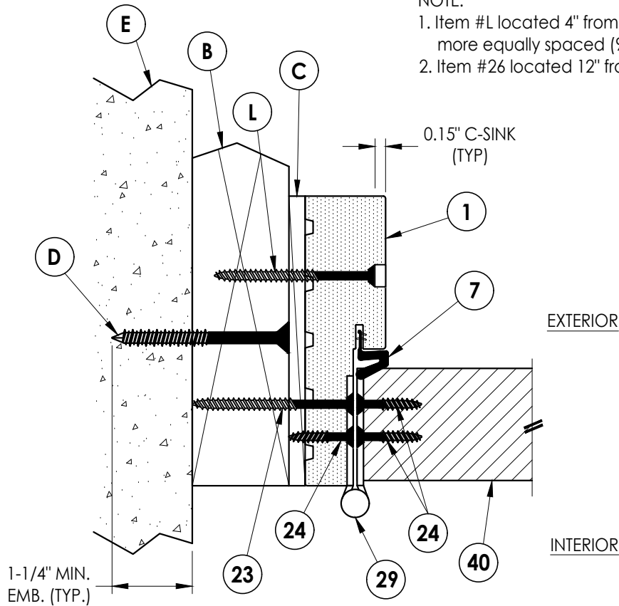
1 HORIZONTAL CROSS SECTION 5 Shown w/ 2X Buck Inswing shown (Outswing similar)
