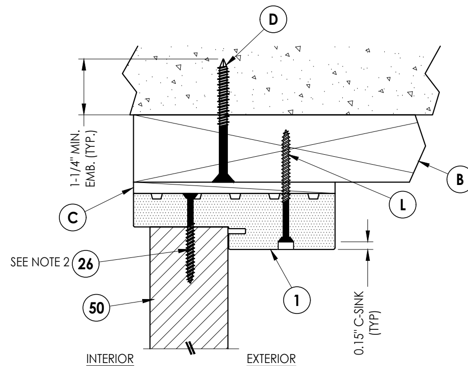
4 VERTICAL CROSS SECTION 5 Shown w/ 2X Buck Inswing shown (Outswing similar)
