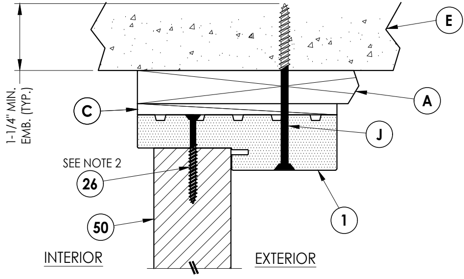
4 VERTICAL CROSS SECTION 6 Shown w/ 1X sub-buck Inswing shown (Outswing similar)
